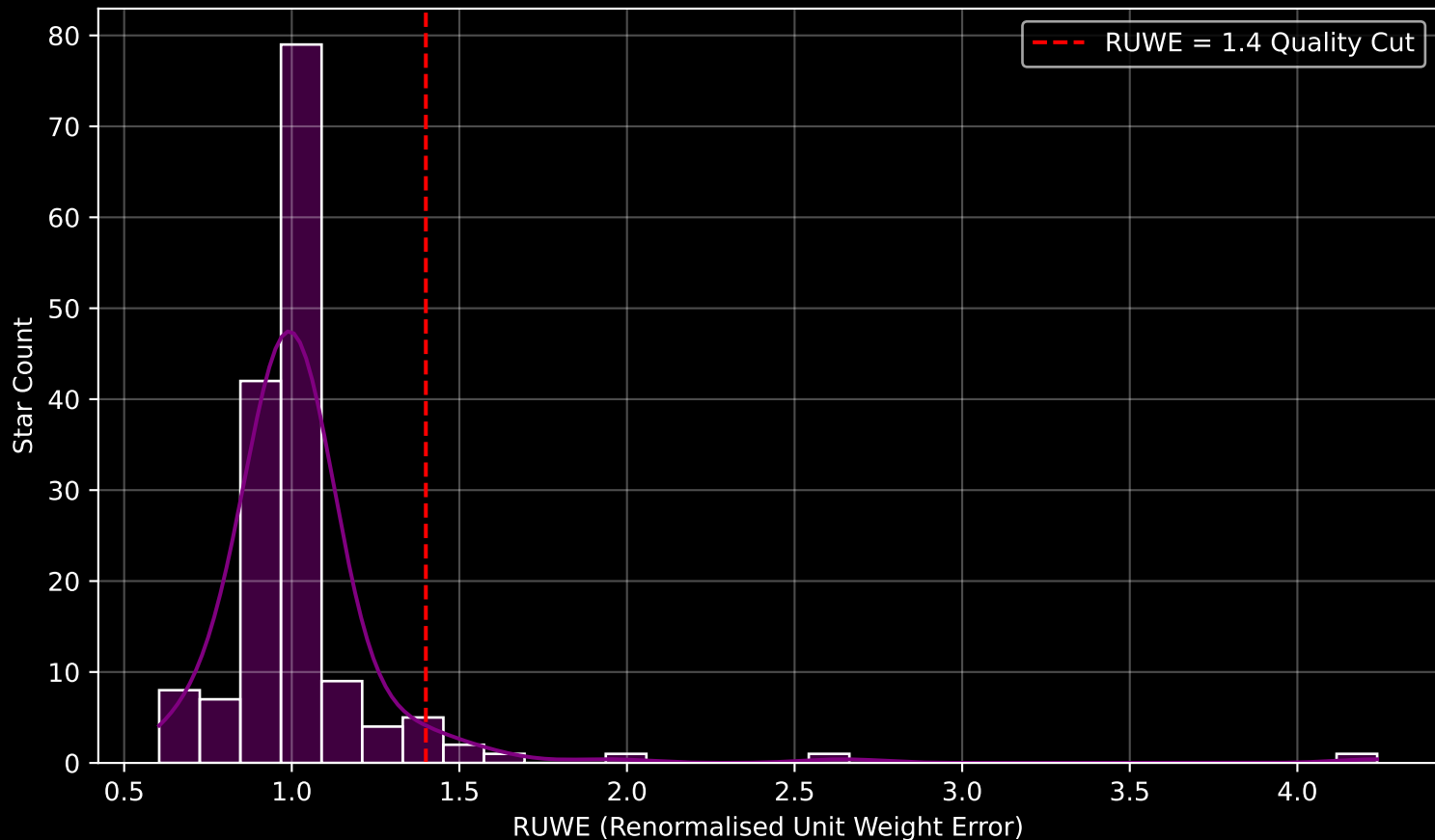
GAPOGEE DR17 Field [K2_C11_359+05_btx] RUWE Distribution (n= 160)
