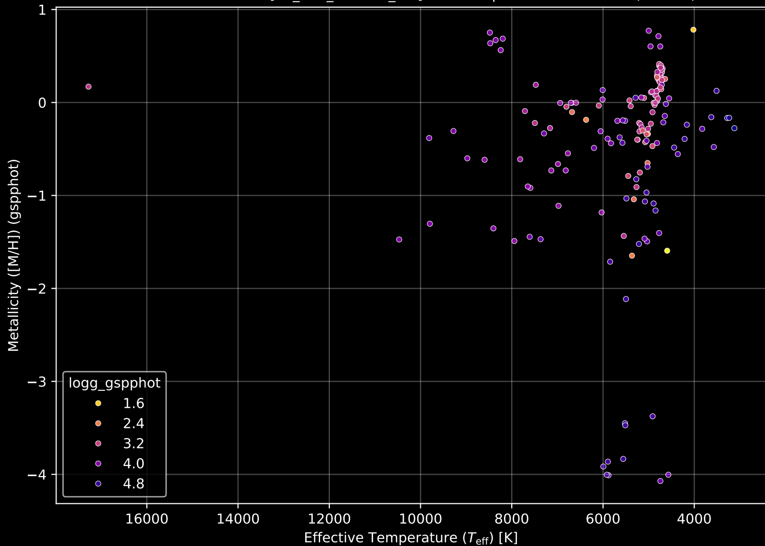
APOGEE DR17 Field: [K2_C11_359+05_btx] Stellar Population Parameters (n= 163)
