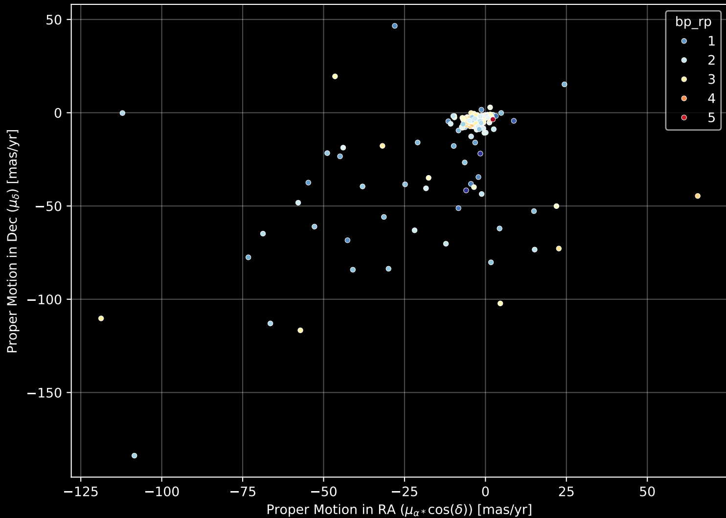
APOGEE DR17 Field: [K2_C11_359+05_btx] Proper Motion Diagram (n= 163)
