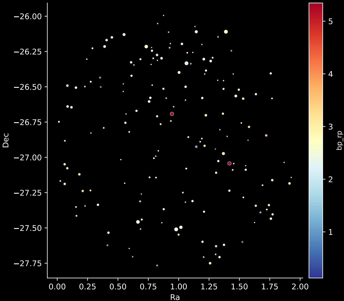
APOGEE DR17 Field: [K2_C11_359+05_btx] Stars: 163
