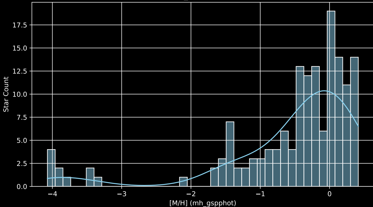
APOGEE DR17 Field: [K2_C11_359+05_btx [M/H] (mh_gspphot) (n= 153)
