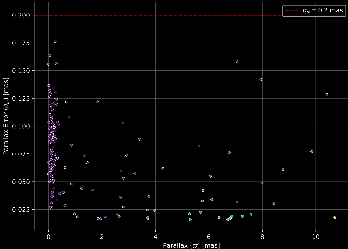
APOGEE DR17 Field: [K2_C11_359+05_btx] Parallax Quality (n= 163)
