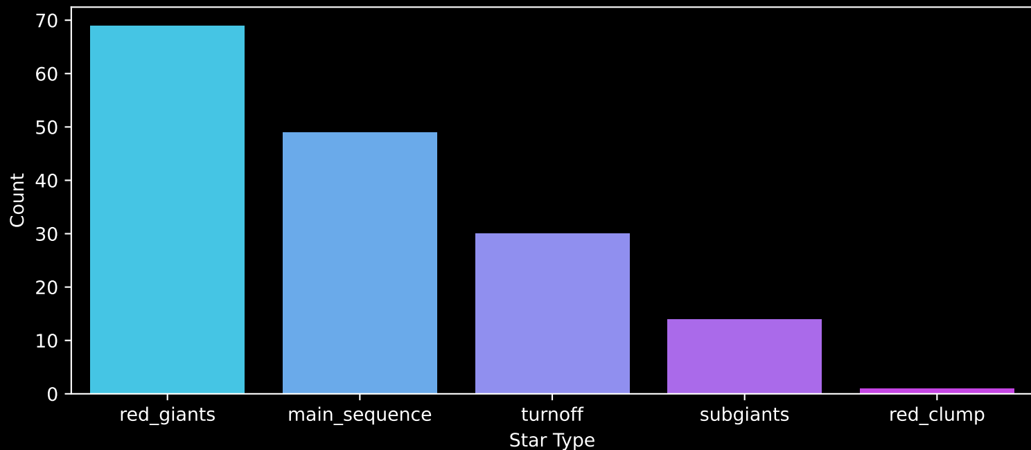
APOGEE DR17 Field: [K2_C11_359+05_btx] Count plot of Star Type
